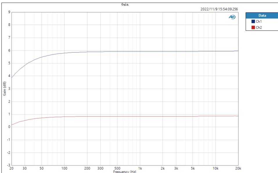
Frequency response (PVDD = 5V, ch1 RIN = 0R, ch2 Rin = 10k)
