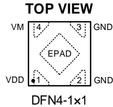
Figure 2. Pin Configuration
